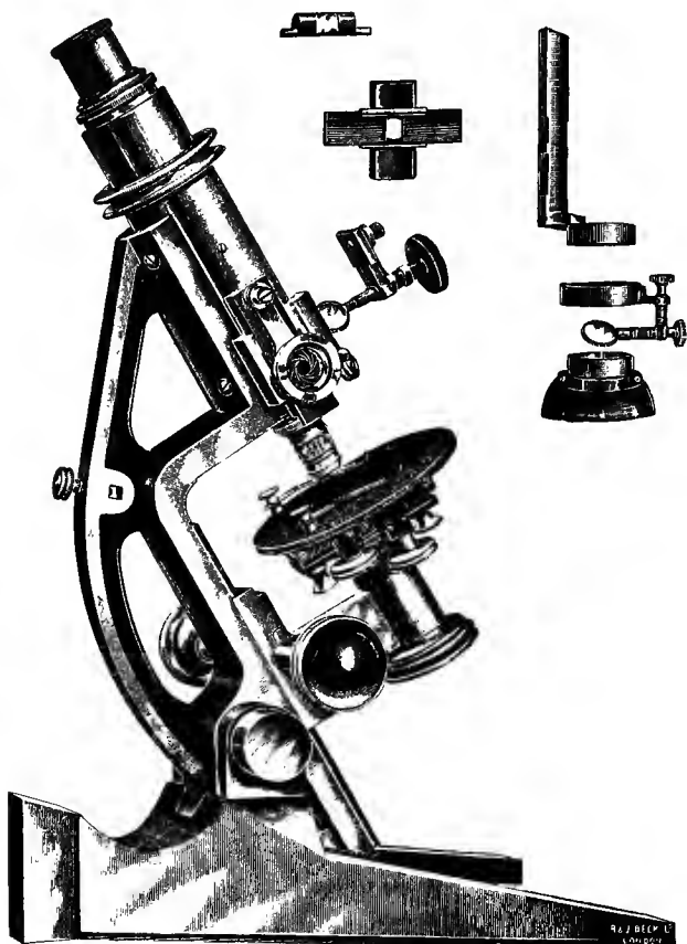
FIG. 64.—Rosenhain microscope.
